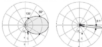
Horizontal Pattern Vertical Pattern 0°–8° electrical downtilt
