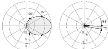
Horizontal Pattern Vertical Pattern 0°–8° electrical downtilt
